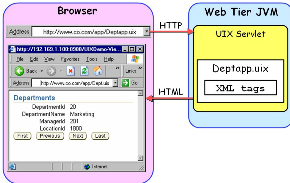
Figure 11. UIX calling sequence
