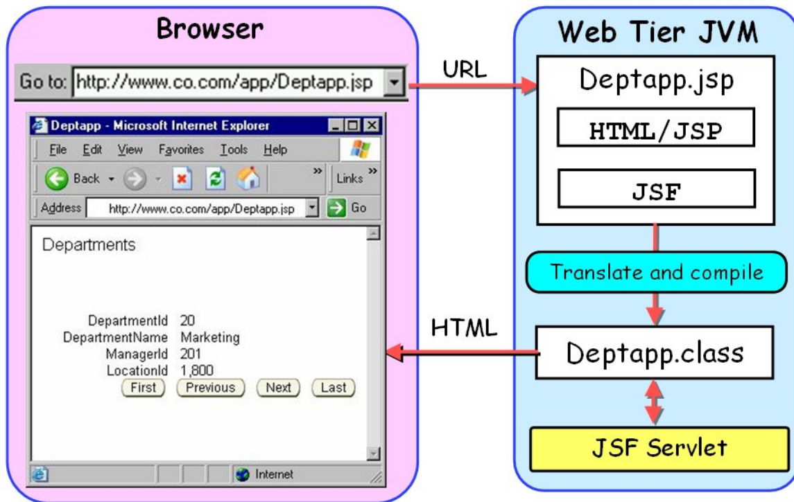
Figure 12. JSF calling sequence
