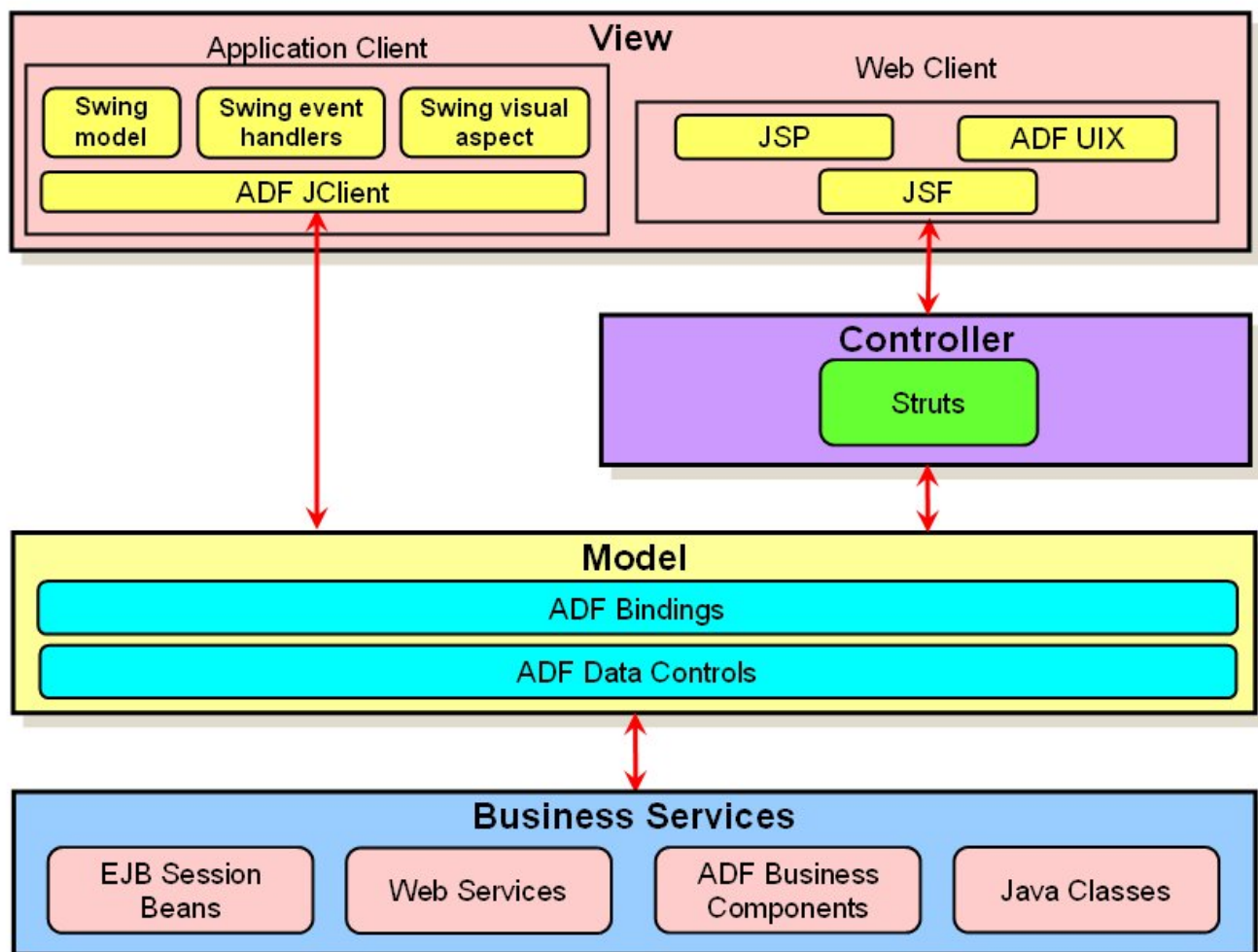
Figure 2. Oracle ADF Technologies
