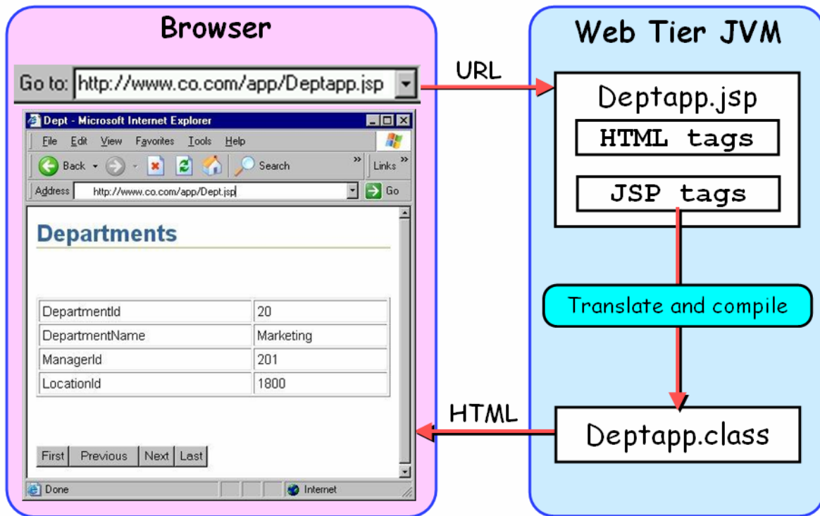
Figure 4. JSP calling sequence
